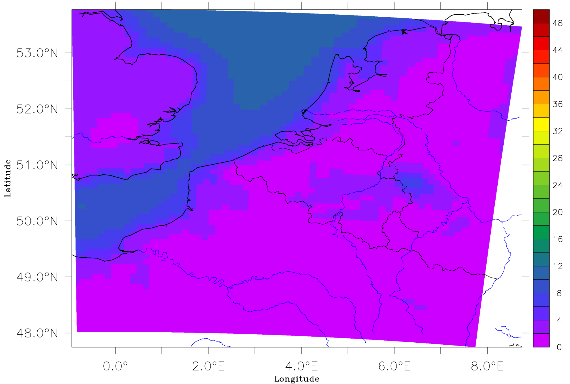
Fig.8 : Percentage of strong wind speed in the last 30 years (in %) >16 m/s
