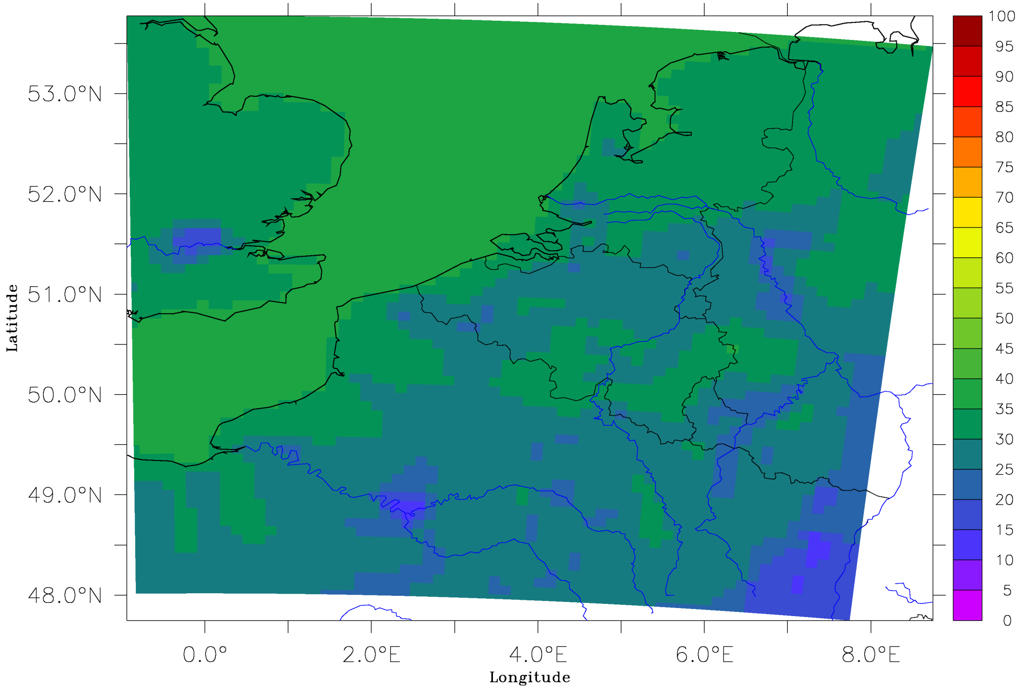
Fig.7 : Percentage of high wind speed in the last 30 years (in %) 8-12 m/s
