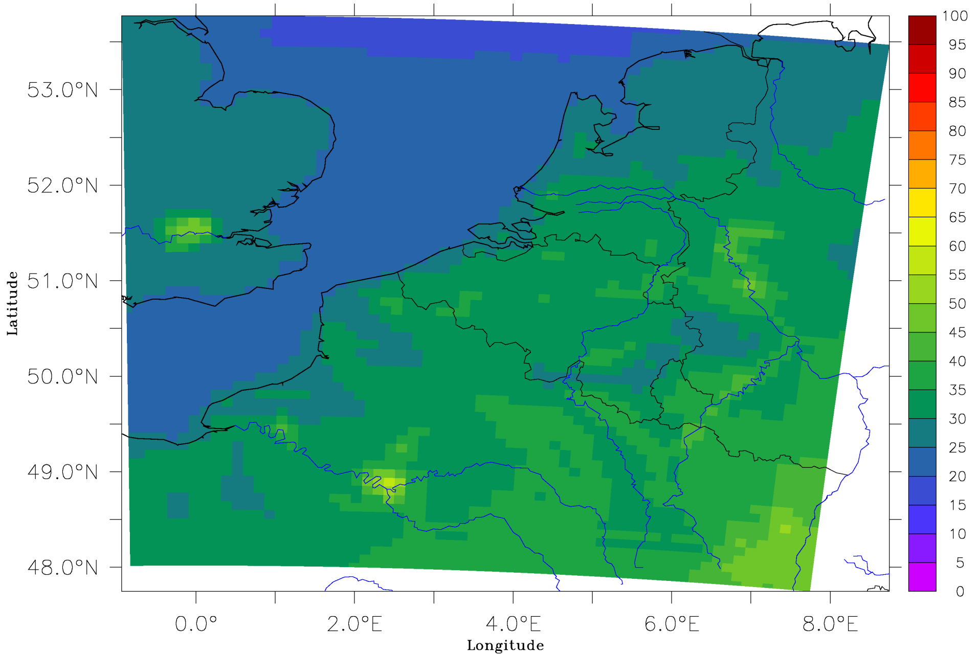
Fig.6 : Percentage of low wind speed in the last 30 years (in %) 0-5 m/s
