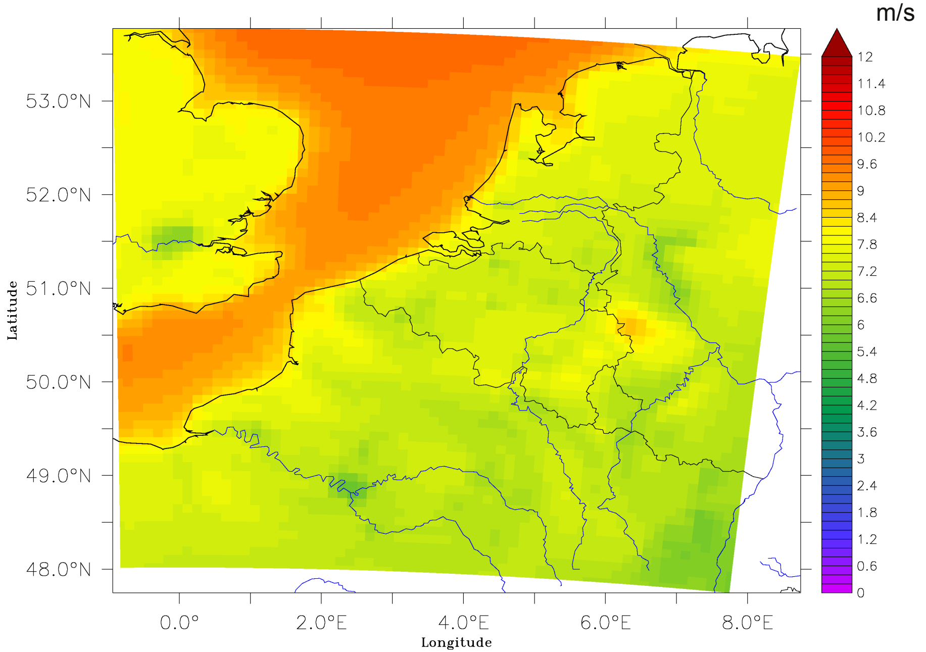
Fig.2 : Mean wind speed in the last 30 years
