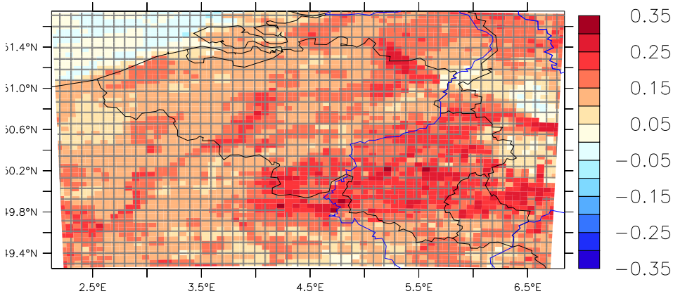
MAR-ERAint (1958-2016)
