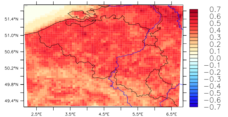
MAR-NORrcp8.5 (2006-2100)
