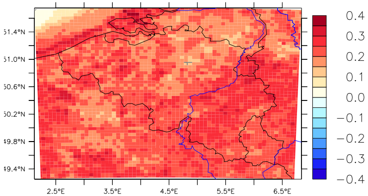
MAR-MIRrcp8.5 (2006-2100)
