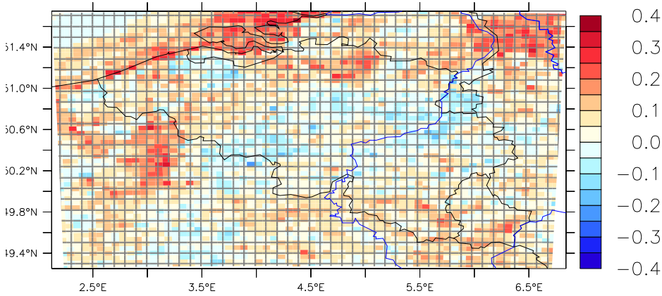
MAR-ERAint (1958-2016)
